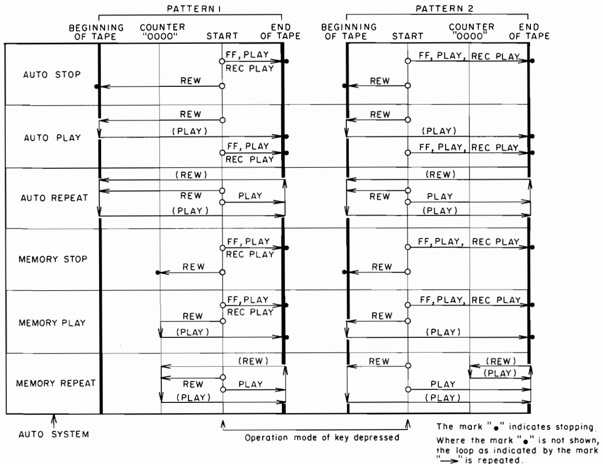
Fig. 52 Auto System Operation
